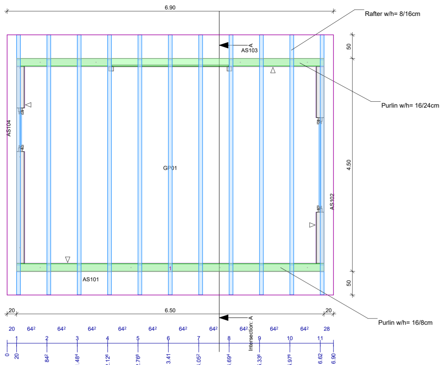
Rafter System
